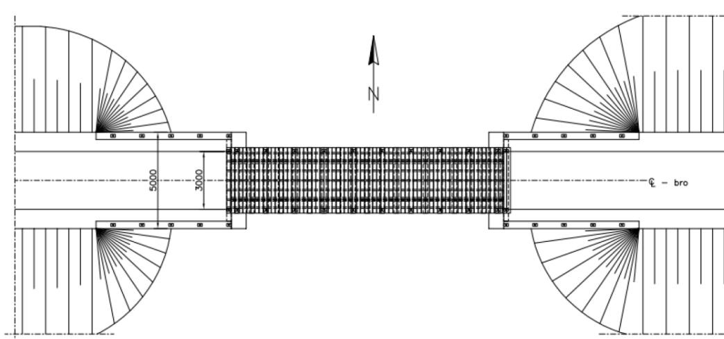
Figur 3. Plan af ny stibro over Stensballe Sund
